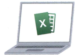
CREATE-SIMPLE
